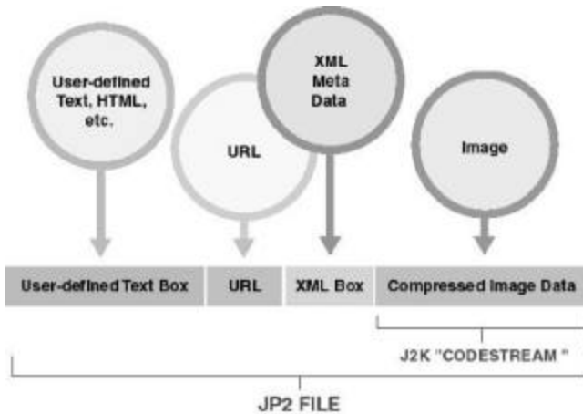
Figure 2: Diagram of typical JP2 file.
